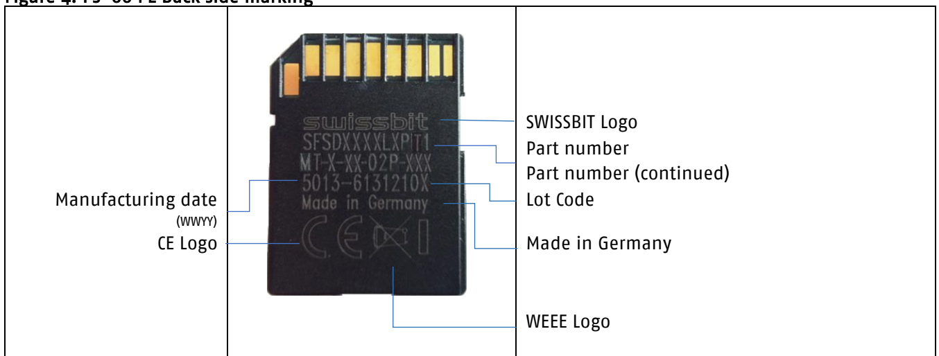
Figure 4: PS-66 PE Back side marking
